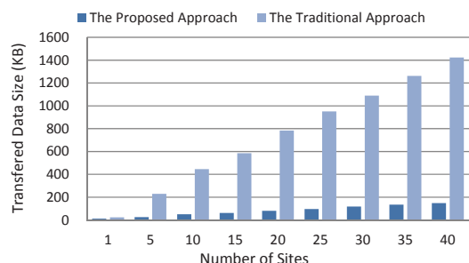
Fig. 21. Network traffic generated between client and servers
