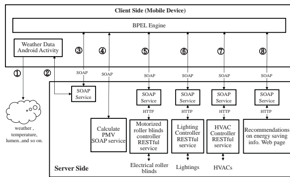
Fig. 3. The heterogeneous service compositions scenario by the traditional approach
