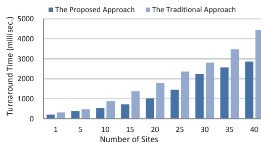
Fig. 16. The turnaround time of invoking motorized roller blinds controller RESTful service
