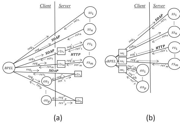
Fig. 13. The network traffic generated between client and server through (a) the traditional framework, and (b) the proposed framework.
