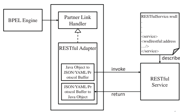
Fig. 6. RESTful adapter architecture
